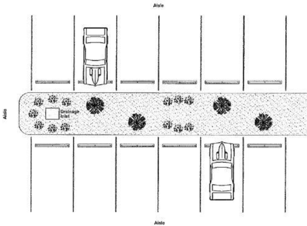
Plan View of Bioswale Island Strip Option
