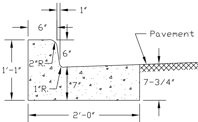
6" CONCRETE CURB
