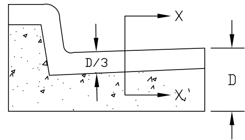
Sawed Contraction Joint
