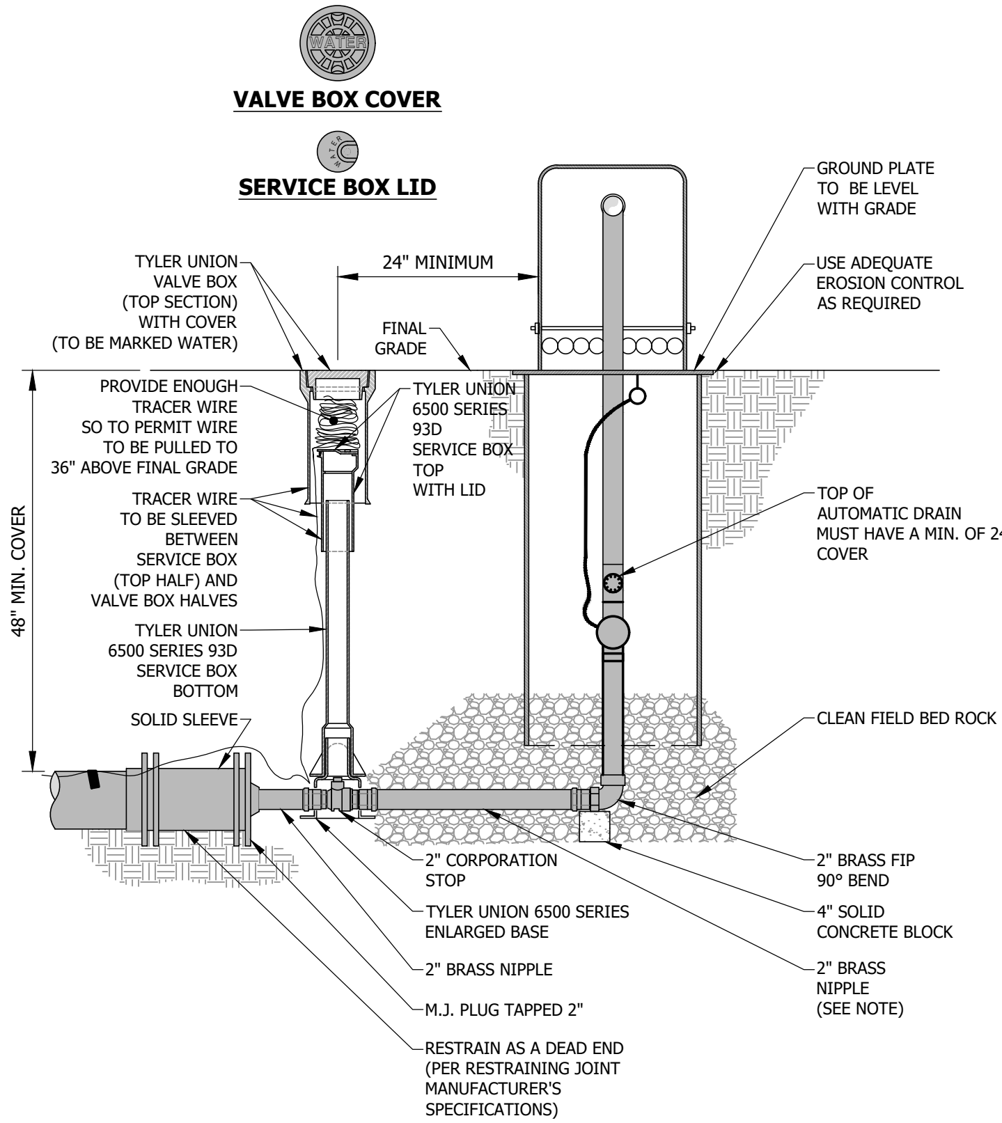
DW35 - AUTOMATIC FLUSHING DEVICE WITH 2" CORPORATION STOP (ECLIPSE 9400)
