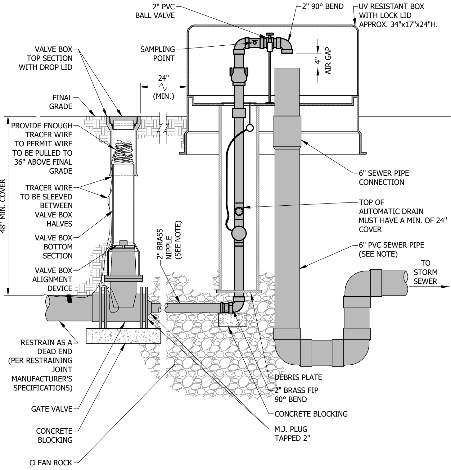
DW33 - AUTOMATIC FLUSHING DEVICE WITH GATE VALVE (ECLIPSE 9800)
