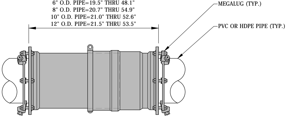
STANDARD UNIT (2.5" MOVEMENT MAX.)
