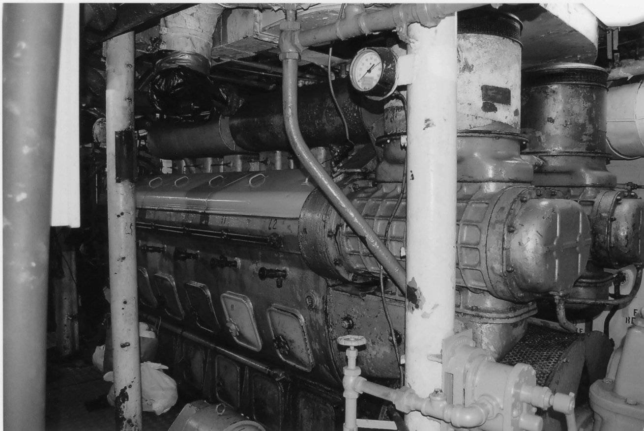
USS LST 325, Evansville vic., Vanderburgh Co., IN #26
